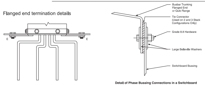
Detail of Phase Bussing Connections in a Switchboard
