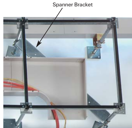
Spanner Bracket
