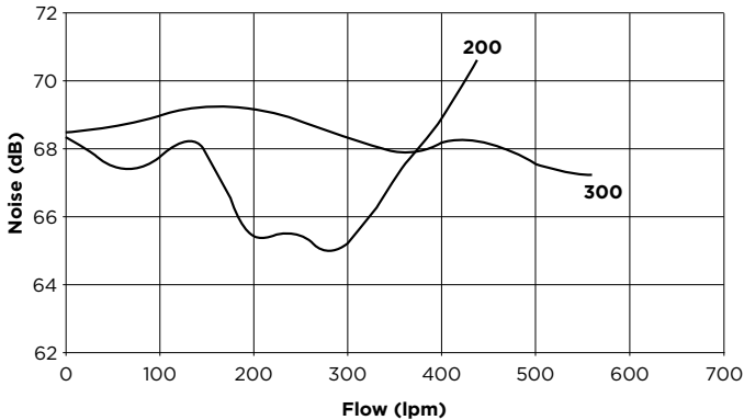
Hydrostar Plus Sound Levels
