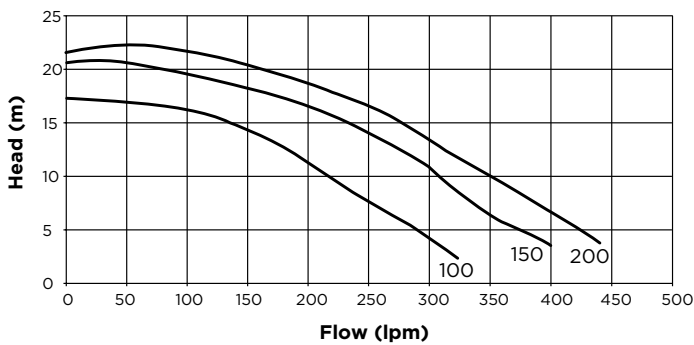
Hydrostorm Flow Curves
