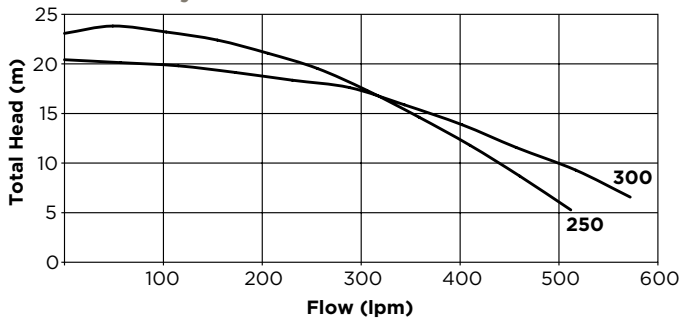
Hydrostorm Plus Flow Curves
