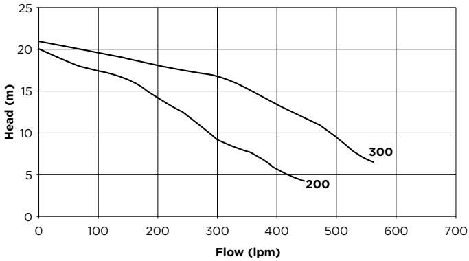
Hydrostar Plus Flow Curves
