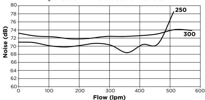
Hydrostorm Plus Sound Levels
