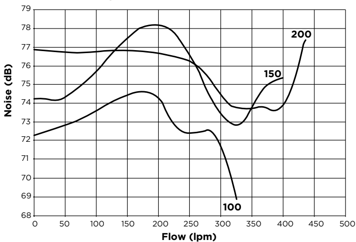
Hydrostorm Sound Levels
